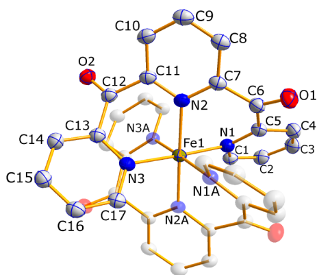
Figure 1. ORTEP drawing of the cation of [\text{Fe}(\text{dcpp})_2](\text{PF}_6)_2 obtained from single-crystal X-ray structure determination. Atoms are represented as 50% probability thermal ellipsoids. Hydrogen atoms and anions are omitted for clarity. Selected bond lengths (Å) and angles (deg): Fe1–N1, 1.985(2); Fe1–N2, 1.974(2); Fe1–N3, 1.989(2); O2–C12, 1.211(2); O1–C6, 1.213(2); N2–Fe1–N1A, 90.48(7); N2–Fe1–N1, 88.79(6); N2–Fe1–N3, 88.87(6); N2–Fe1–N3A, 91.86(6); N1–Fe1–N1A, 90.61(9); N1–Fe1–N3A, 89.07(7); N3–Fe1–N3A, 91.35(9); N1–Fe1–N3, 177.63(6); N2–Fe1–N2A, 178.96(8). Symmetry code A: -x, y, -z + 1/2 . 14
