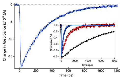
Figure 2. Time-resolved electronic absorption data for [\text{Fe}(\text{bpy})_3](\text{PF}_6)_2 (red, inset), [\text{Fe}(\text{terpy})_2](\text{PF}_6)_2 (black, inset), and [\text{Fe}(\text{dcpp})_2](\text{PF}_6)_2 (blue) in room temperature CH 3 CN solutions following excitation near the maximum of each compound's ^1\text{A}_1 \rightarrow ^1\text{MLCT} visible absorption feature. The solid lines correspond to fits of the data to single-exponential kinetic models with time constants of 0.96 \pm 0.02 , 5.35 \pm 0.15 , and 0.28 \pm 0.01 ns, respectively.
